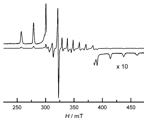
Figure 5. X-band EPR spectrum of 2 measured at 77.4 K on a chilled \text{CH}_2\text{Cl}_2/\text{CH}_2\text{ClCH}_2\text{Cl} (1:1) solution. EPR spectra of polycrystalline samples are given in Figure S2 in the Supporting Information.
