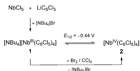
Scheme 1. Succinct synthetic procedures to obtain compounds 1 and 2 with indication of their electrochemical relationship ( E_{1/2} potential given vs. SCE).
