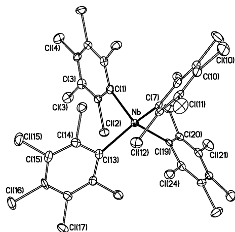
Figure 1. Thermal ellipsoid diagram (50% probability) of the [\text{Nb}^{\text{III}}(\text{C}_6\text{Cl}_5)_4]^- anion in 1 . Secondary ortho -Cl...Nb interactions with average Nb...Cl = 304.2(1) pm are not drawn for clarity. Selected bond length [pm] and angles [°] with estimated standard deviations: average Nb–C 222.8(4); C(1)–Nb–C(7) 111.45(14), C(1)–Nb–C(13) 98.89(13), C(1)–Nb–C(19) 117.63(14), C(7)–Nb–C(13) 116.03(13), C(7)–Nb–C(19) 101.66(12), C(13)–Nb–C(19) 111.98(13).
