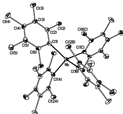
Figure 2. Thermal ellipsoid diagram (50% probability) of the neutral species [\text{Nb}^{\text{IV}}(\text{C}_6\text{Cl}_5)_4] in 2 . Secondary ortho -Cl...Nb interactions with Nb...Cl = 299.8(1) pm are not drawn for clarity (cf. Figure 3). Selected bond length [pm] and angles [°] with estimated standard deviations: Nb–C(1) 218.2(3); C(1)–Nb–C(1A) 115.70(8), C(1)–Nb–C(1B) 97.62(15), C(1)–Nb–C(1C) 115.70(8), C(1A)–Nb–C(1B) 115.70(8), C(1A)–Nb–C(1C) 97.62(15), C(1B)–Nb–C(1C) 115.70(8).
