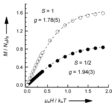
Figure 4. Dependence of M/\mu_B N_A on \mu_B H/k_B T for compounds 1 (○) and 2 (●) measured at 1.8 K. The dashed lines correspond to the Brillouin functions best matching the experimental data in each case. Data obtained at 5 and 78 K (not shown for clarity) overlap with those given here.
