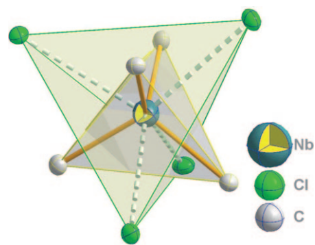
Figure 3. Local coordination environment of the \text{Nb}^{\text{IV}} center in 2 . 2\cdot 2\text{C}_6\text{H}_{14} (thermal ellipsoid diagram with 50% probability) with indication of the inner \text{NbC}_4 and outer \text{NbCl}_4 tetrahedra. Secondary ortho -Cl...Nb interactions are indicated with broken lines.
